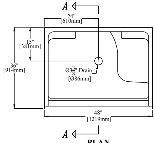
48" [1219mm] Shower w/ 8" [203mm] Threshold, Molded Seat CENTER DRAIN Left Hand Version (5843L/S) Shown
